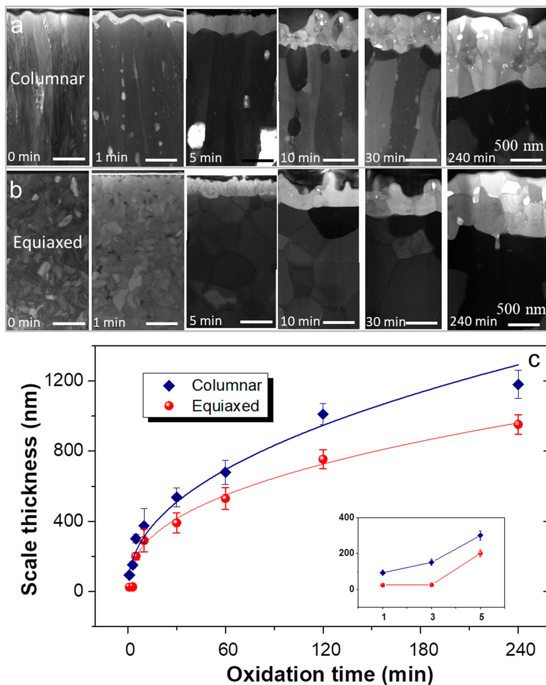
Figure 2. (a-b) STEM bright field images (Helios) of the cross-sections of columnar (a) and equiaxed (b) grained Cr 2 AlC coatings before oxidation and after oxidation at 1100°C from 1 to 240 min. The measured scale thickness is plotted as a function of oxidation time for each sample. (c) Variation of the oxide scale thickness with oxidation time and corresponding power law fit in the equiaxed and columnar grained samples. The inset in (c) shows the initial scale thickness from 1 to 5 min.
